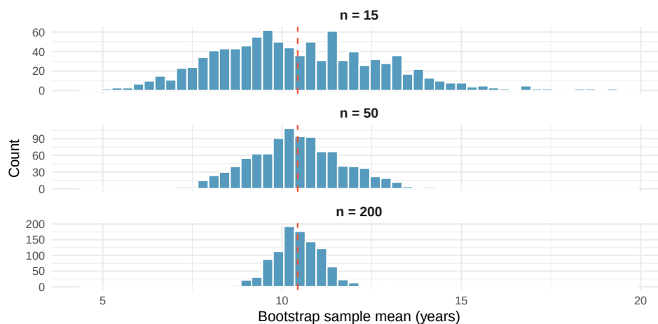
Figure 31: The effect of sample size on the bootstrap distribution. Larger samples produce narrower bootstrap distributions, leading to narrower confidence intervals. All three panels use the same population of penny ages.
