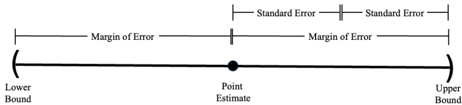
Figure 27: Diagram of the relationship between the 95% confidence interval, margin of error, and standard error.
