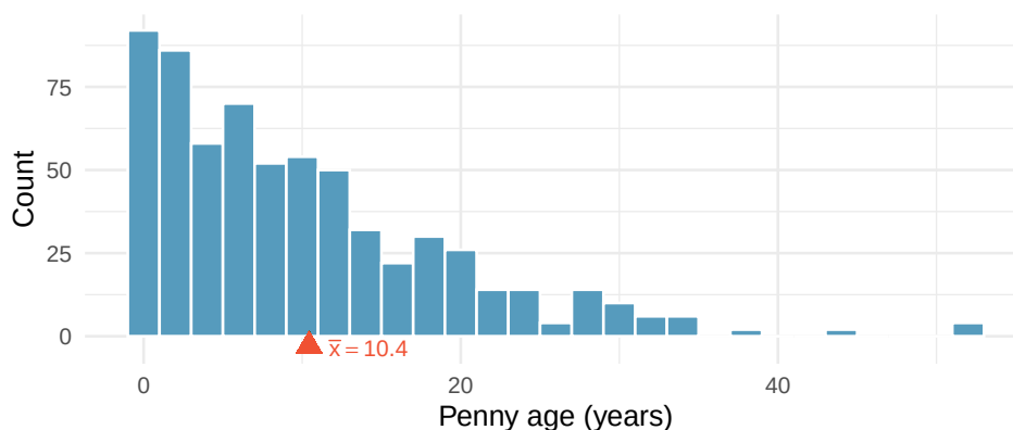
Figure 28: Distribution of ages for 648 pennies sampled from circulation. The distribution is right-skewed with a mean of about 10.4 years. The sample mean is marked with a red triangle. Open in StatLens
