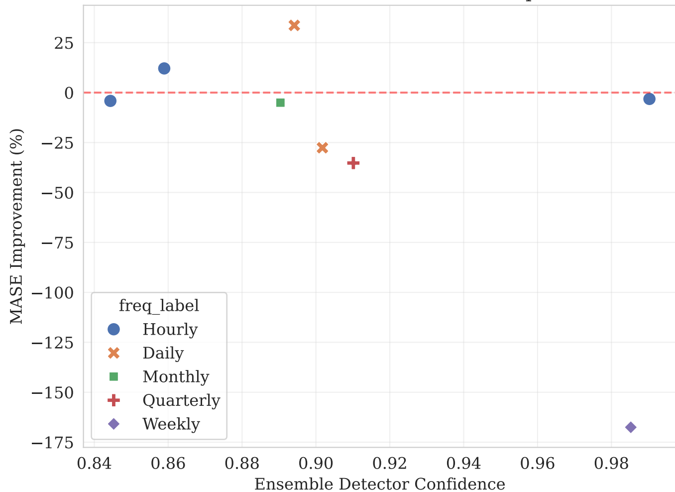
Detector Confidence vs. Performance Improvement
