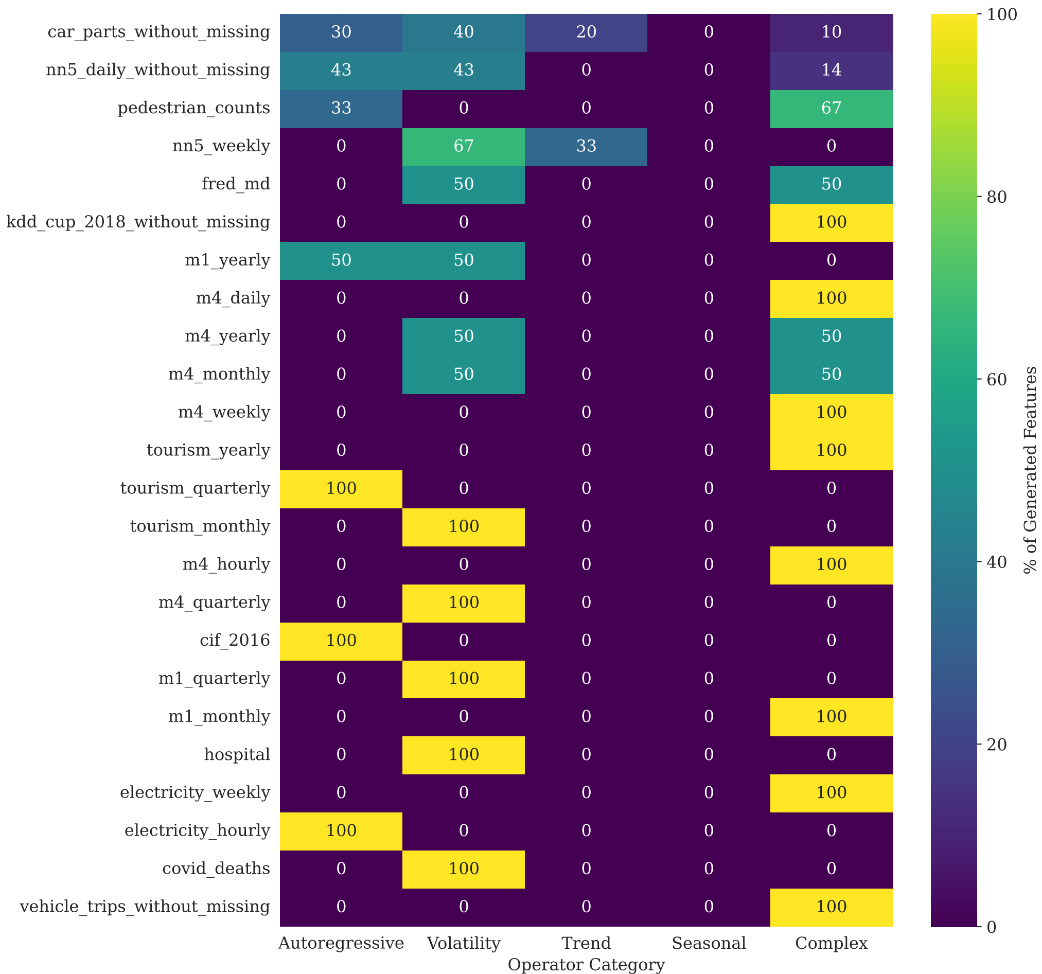
Feature Discovery Profile (Auto Ensemble)
