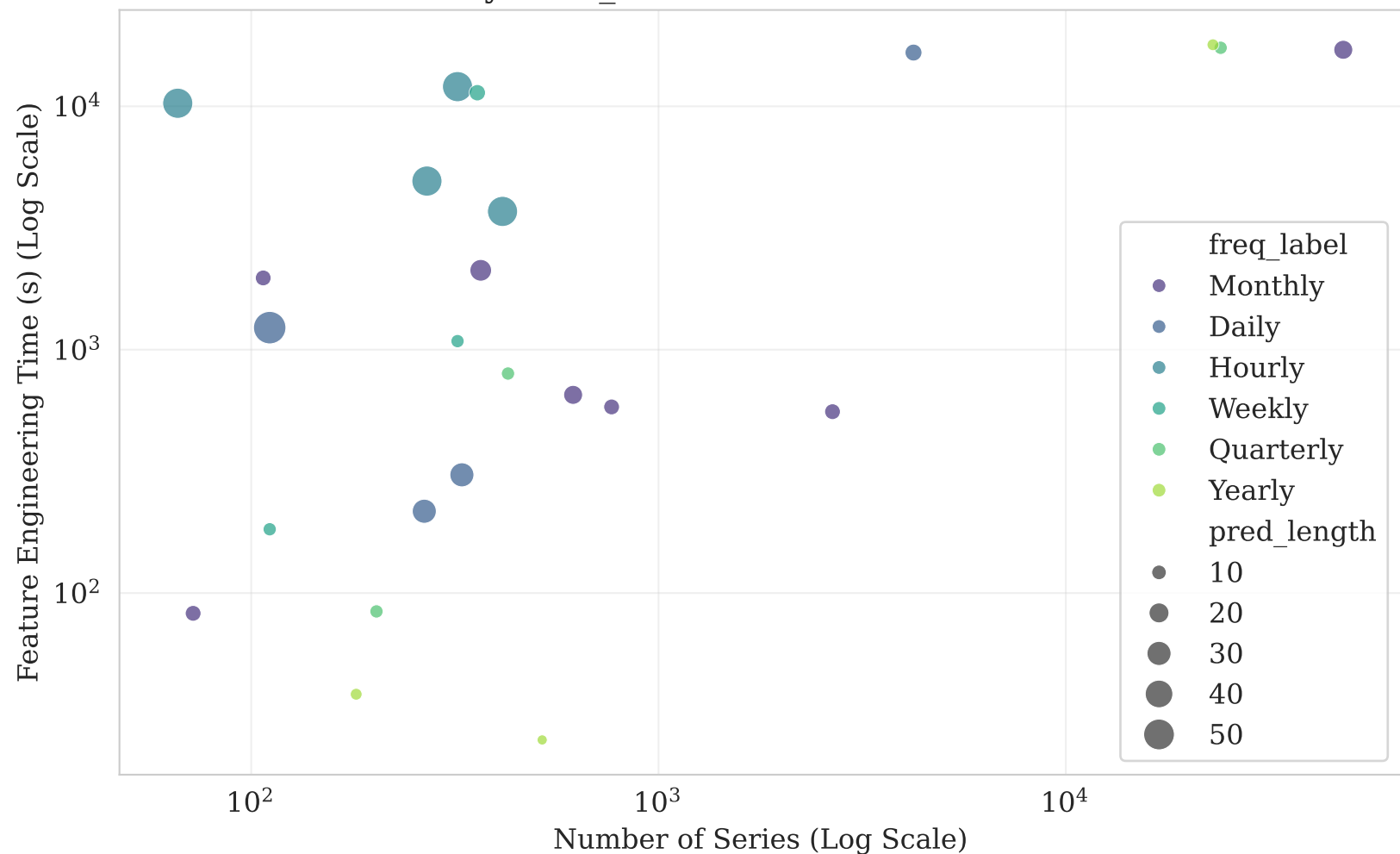
Scalability: auto_ensemble Runtime vs Dataset Size
