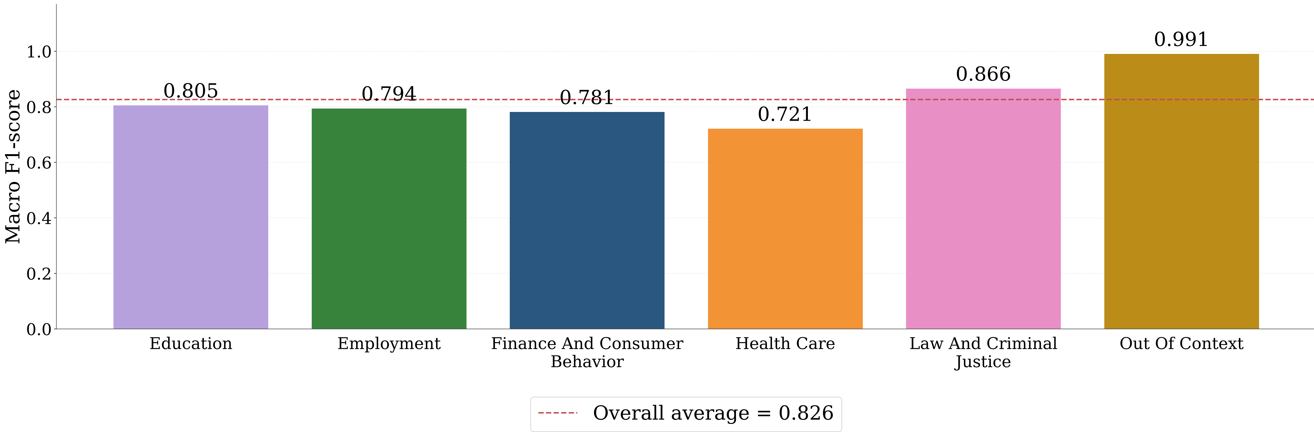
Average Macro F1-score by Dataset Category
