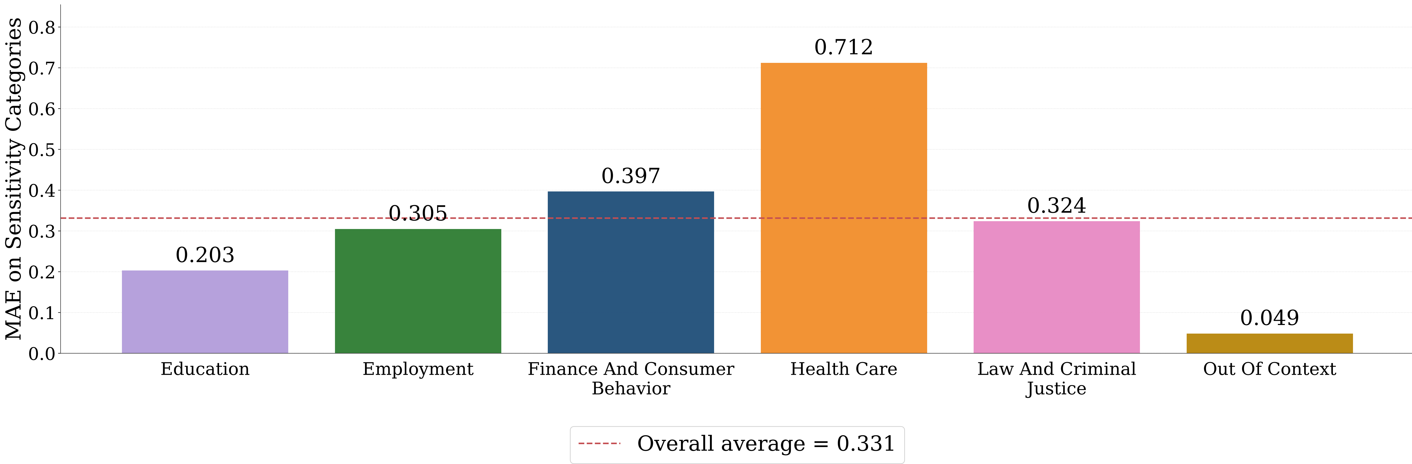
Average MAE Category by Dataset Category
