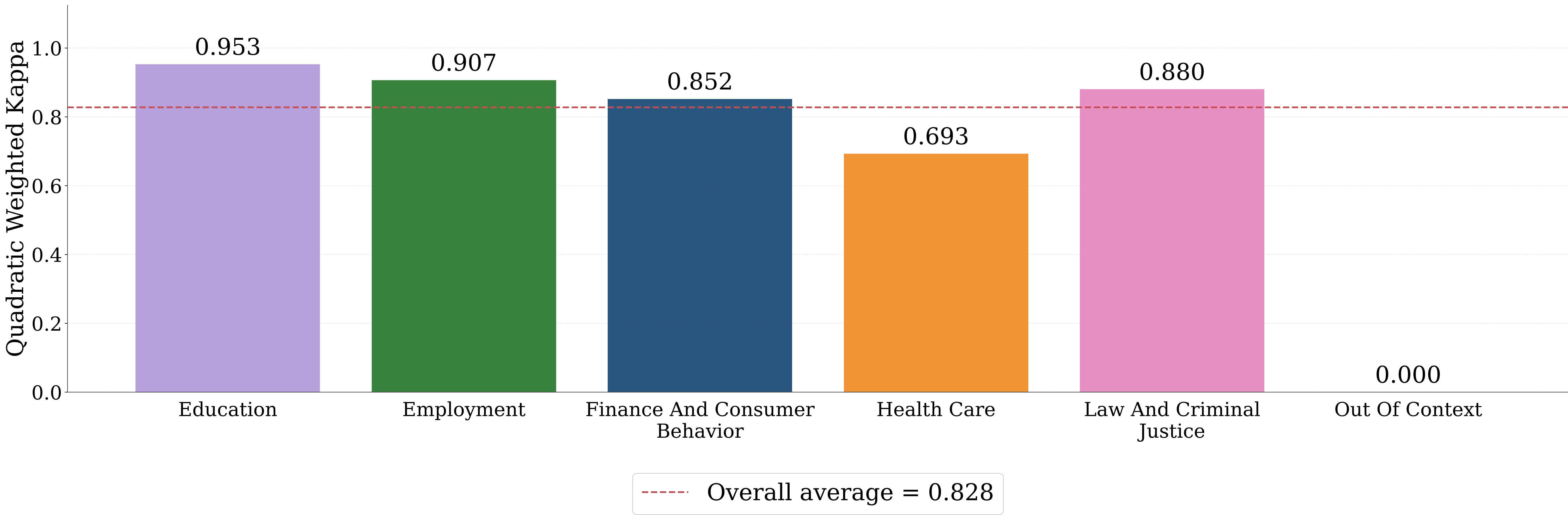
Average Quadratic Weighted Kappa by Dataset Category
