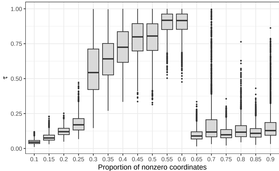
Collapse of the horseshoe global scale
