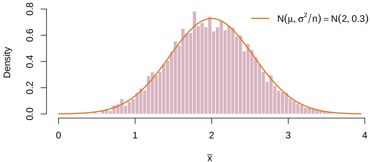
Sampling distribution of \bar{X}_{30} from N(2,9)
