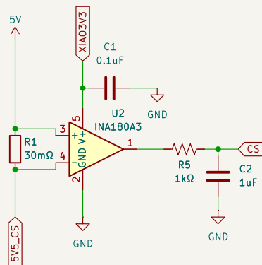
CURRENT SENSE
