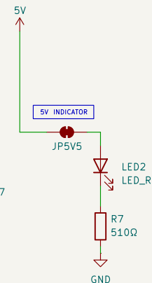
LED
