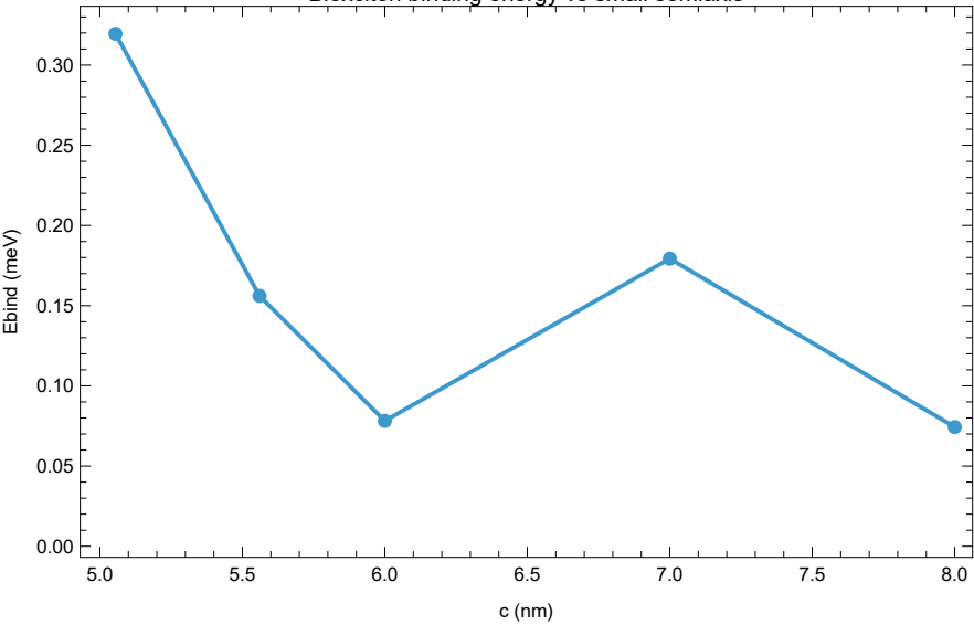
Biexciton binding energy vs small semiaxis
