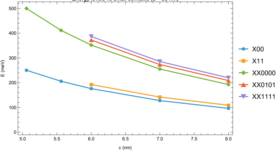
Energy levels vs small semiaxis ( a = 50 nm)
