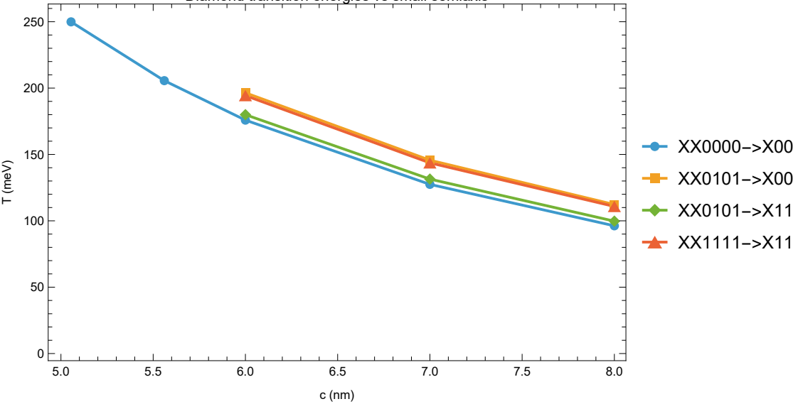
Diamond transition energies vs small semiaxis
