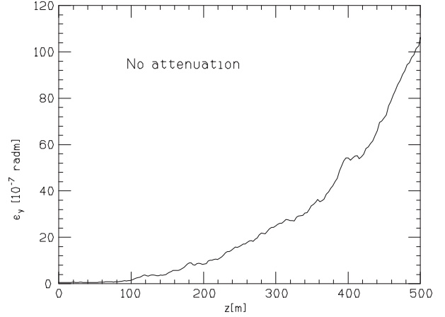
Figure 1: 2nd bunch emittance-growth without RFQs.
