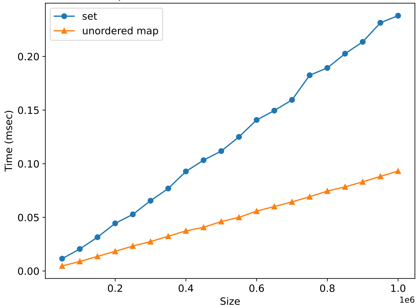
Comparison of set and hash table insert() times
