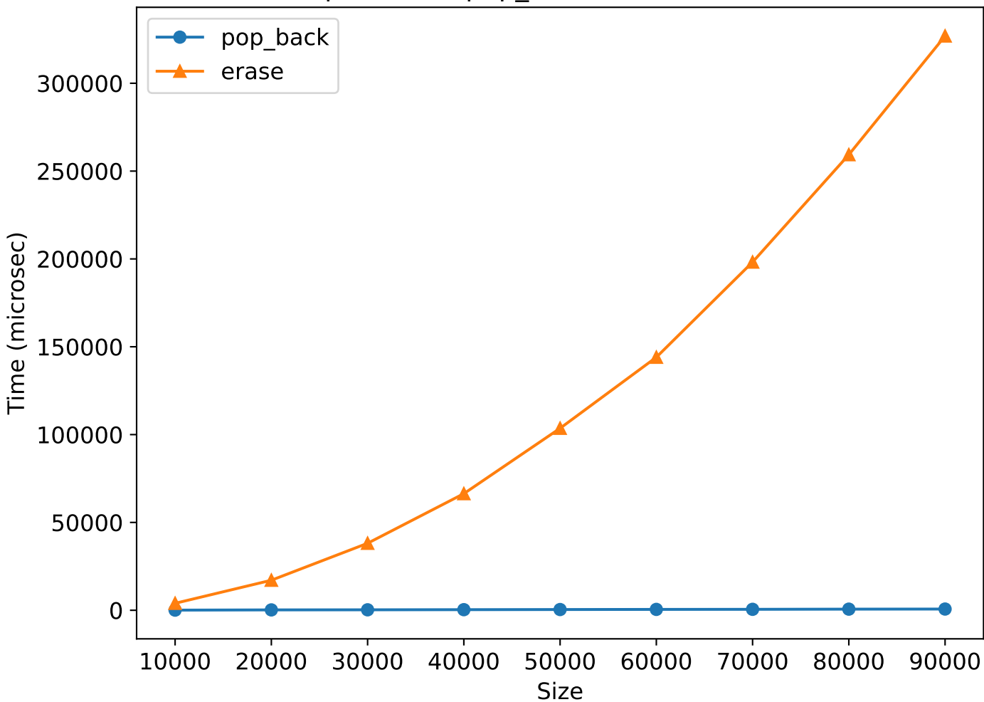
Comparison of pop_back() and erase() times
