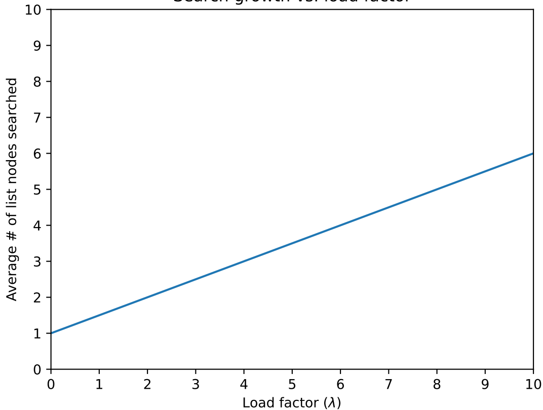
Search growth vs. load factor
