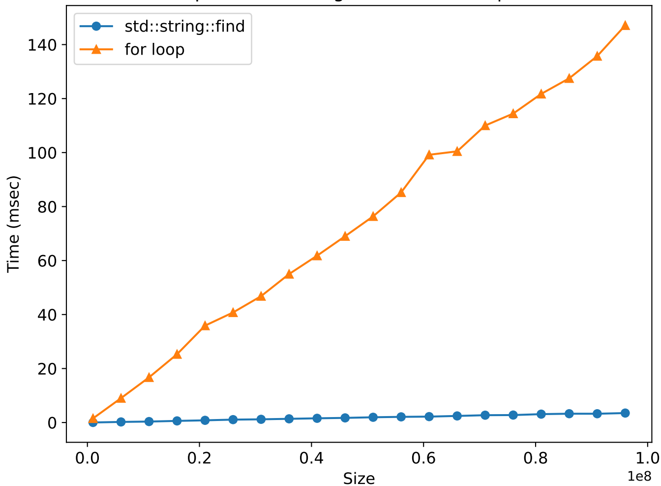
Comparison of string::find and for loop times
