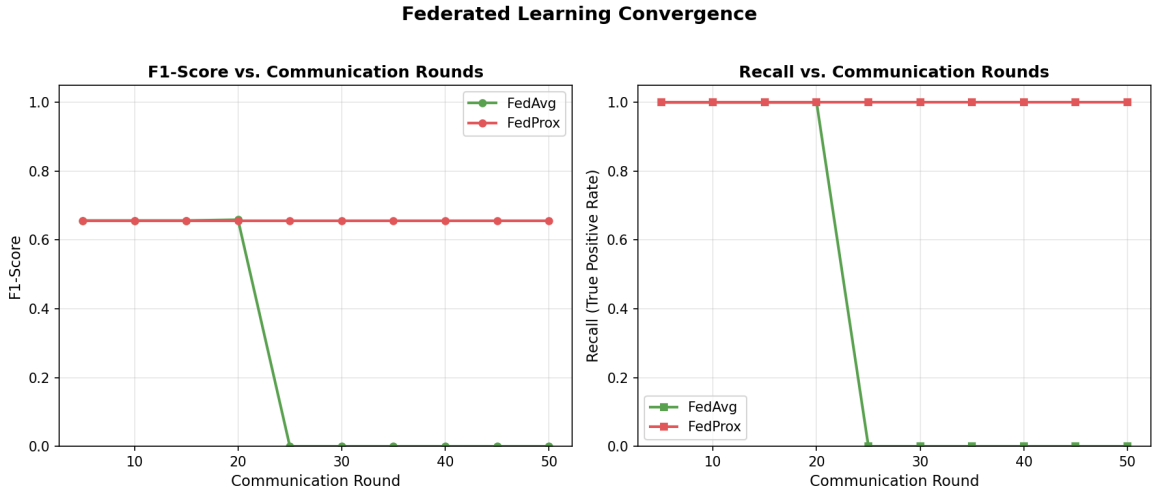
Figure 4: Validation-monitored convergence over 50 rounds: per-round validation F_1 (left panel) and validation Recall (right panel) at the development threshold, as evaluated by the shipped server-side path (FedAvg vs FedProx; ROC-AUC values quoted in the text come from the round-level validation history in the run artefacts, not from this figure). Plain FedAvg’s evaluated F_1 collapses toward zero after round 20 while its recall saturates at 1.0 (the all-positive degenerate regime); FedProx ( \mu=0.01 ) holds its monitored statistics throughout. Section 6.9 shows this trajectory measures normalisation compatibility, not information content: the same FedAvg weights carry \sim 0.95 test ROC-AUC under correct normalisation at every round.
