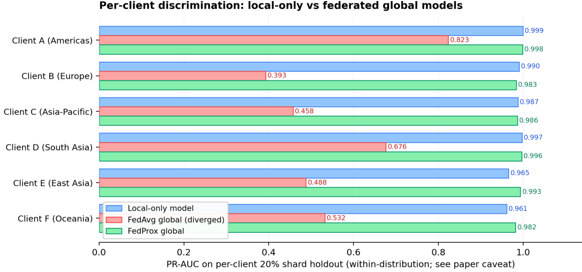
Figure 7: Per-client PR-AUC of local-only models versus the federated global models, evaluated on a held-out 20% slice of each client’s shard (neutral client labels; no real institution participates). Caveat: the federated models trained on the full shards, so their holdout scores are within-distribution rather than clean generalisation estimates (see Section 8).
