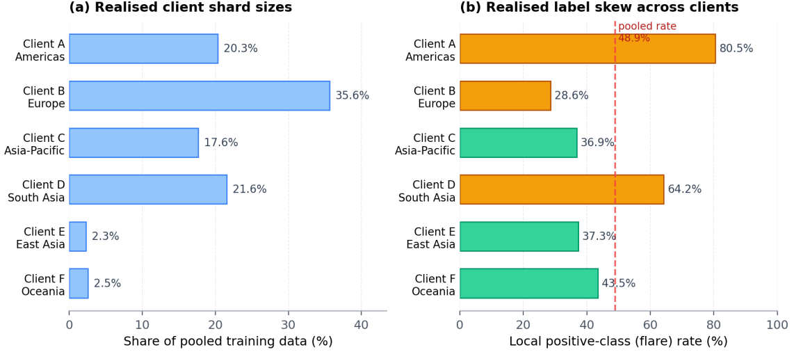
Figure 2: Non-IID partitioning of the pooled, class-balanced training data into six regional clients by label-aware Dirichlet sampling (concentration \alpha = 1.0 , RNG seed 42, Section 4); proportions are read directly from the frozen run’s cached client assignment. (a) Realised relative shard sizes. (b) Realised local flare rates against the pooled rate of 48.9%: label skew spans 28.6%–80.5%, emulating observatories that monitor very different active-region populations.
