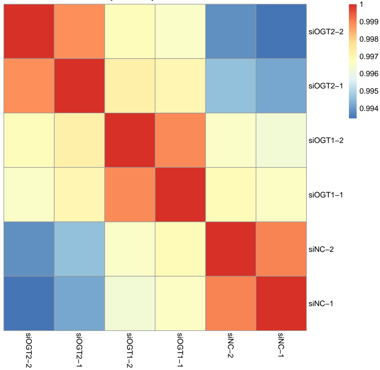
Sample-Sample Correlation
