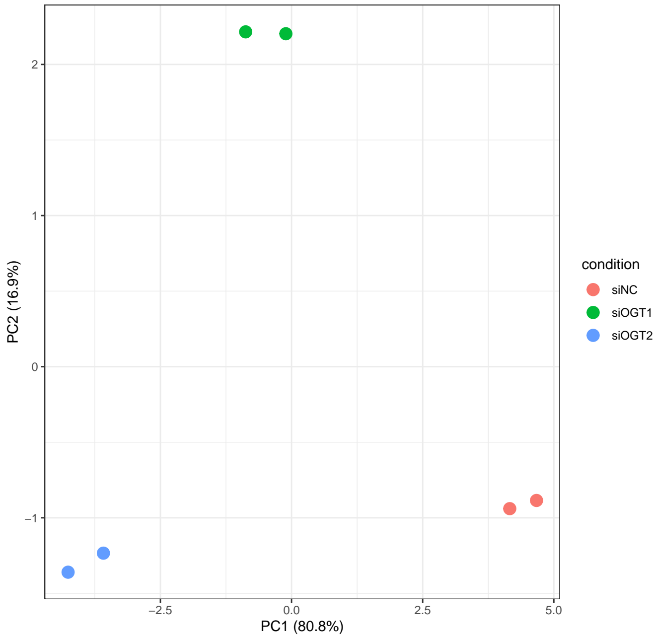
PCA of top 500 most variable genes
