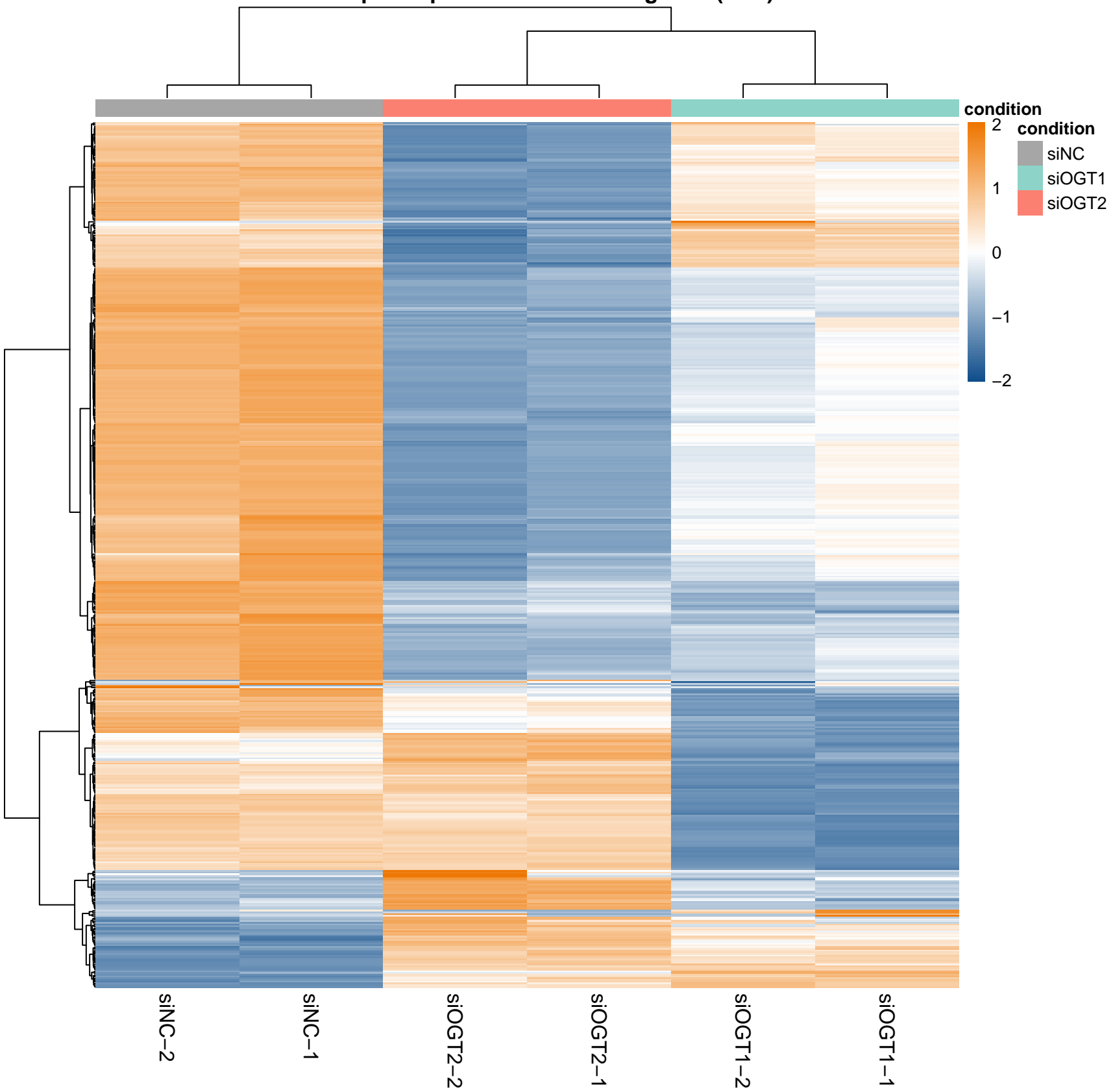
Heatmap of top 500 most variable genes (VST)
