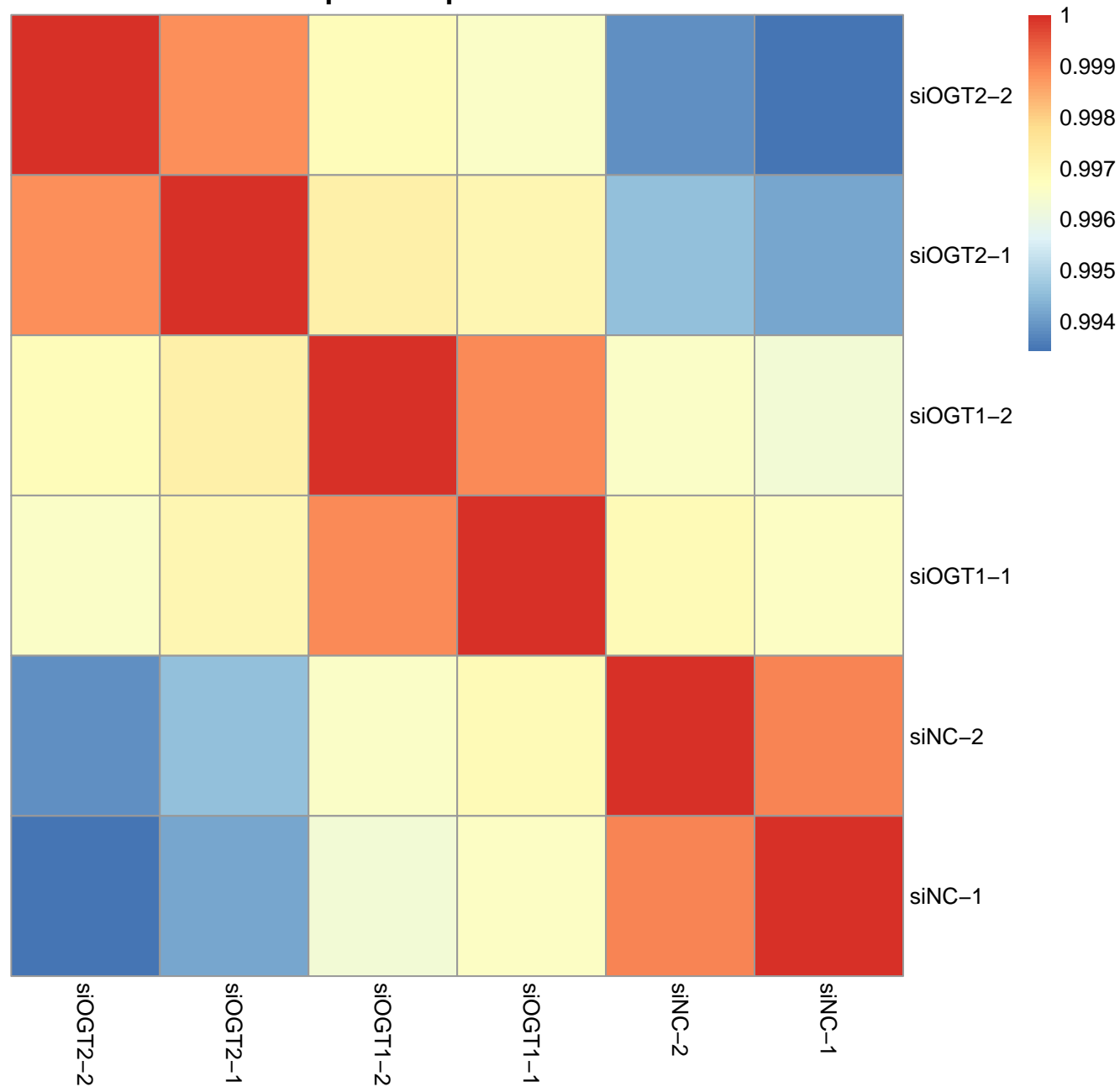
Sample-Sample Correlation
