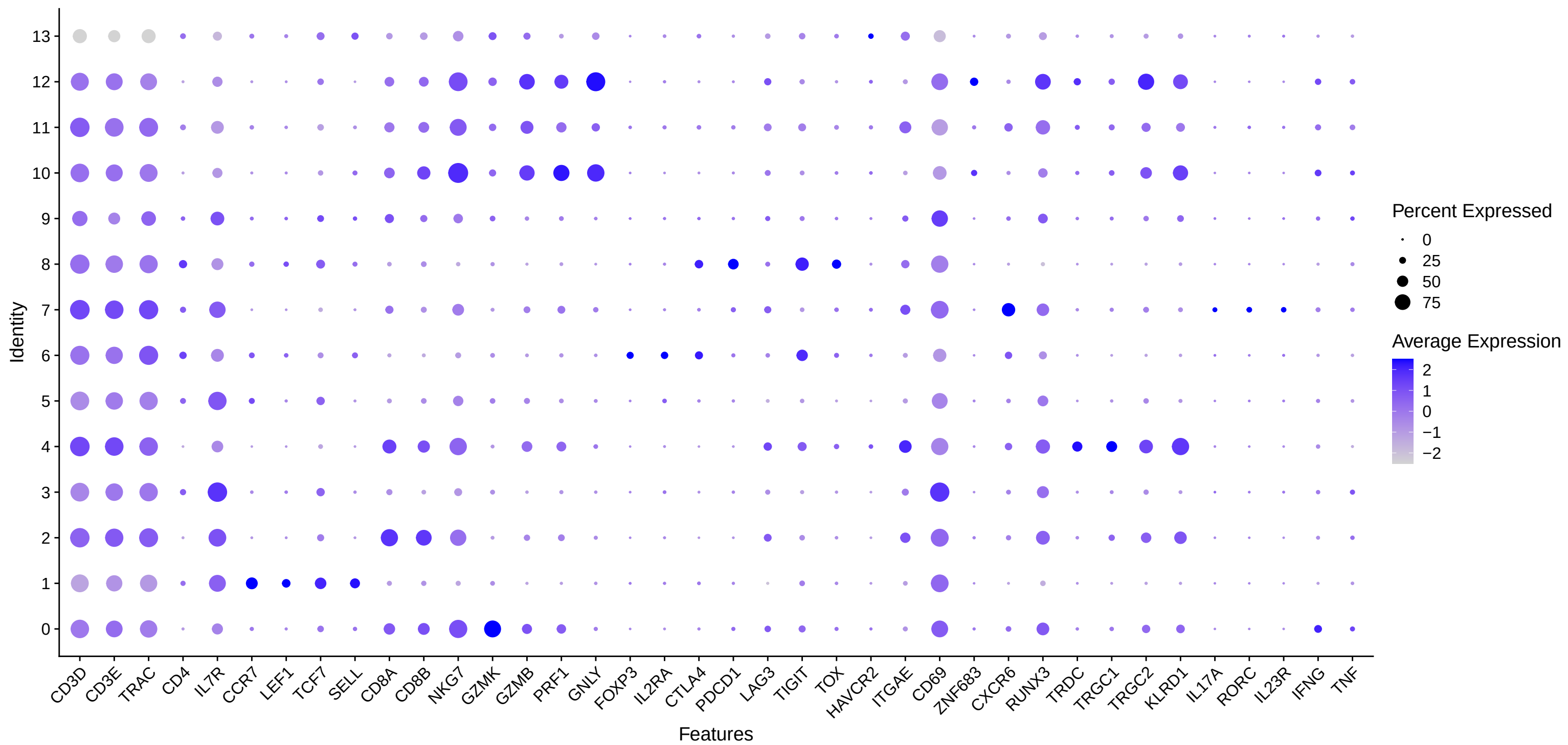
Canonical Immune Marker Expression Across Seurat Clusters
