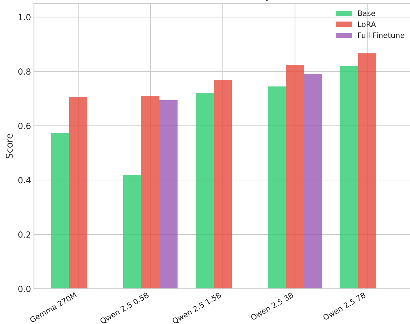
Abstain Accuracy
