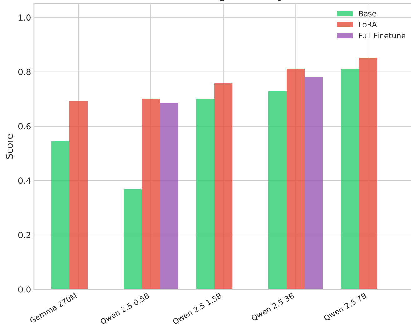
Abstain Accuracy
