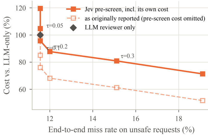
Fig. 5. Two-tier safety review (Jev pre-screen → LLM reviewer): cost vs. end-to-end miss rate over thresholds \tau . Dashed: the original accounting, which omitted the pre-screen’s own cost.
