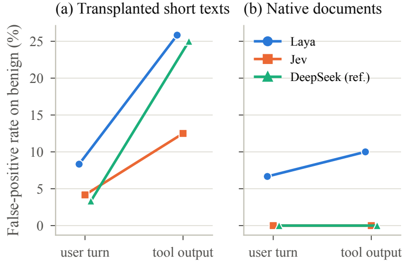
Fig. 6. Benign false-positive rate of injection detectors by delivery channel. (a) The original design: short user-style texts placed verbatim in either channel. (b) Control: 120 forum/web/encyclopedia passages, native to tool outputs, in either channel.
