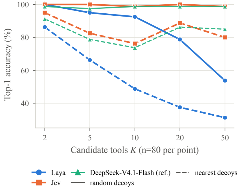
Fig. 2. Tool selection vs. number of candidates. Solid: random distractors (track B). Dashed: nearest-neighbour distractors (B2).
