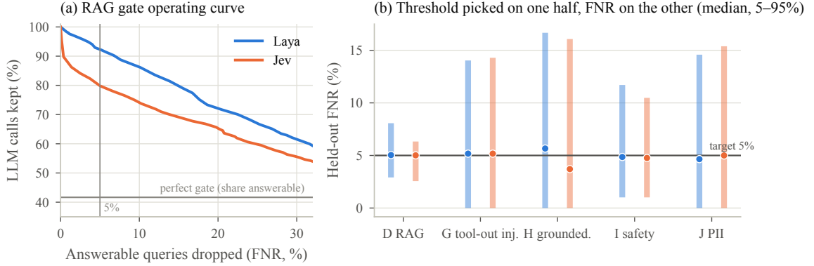
Fig. 4. (a) RAG gate: share of LLM calls kept vs. answerable queries dropped (in-sample). (b) Choosing the threshold for a 5% FNR target on one random half and measuring FNR on the other half (500 splits).
