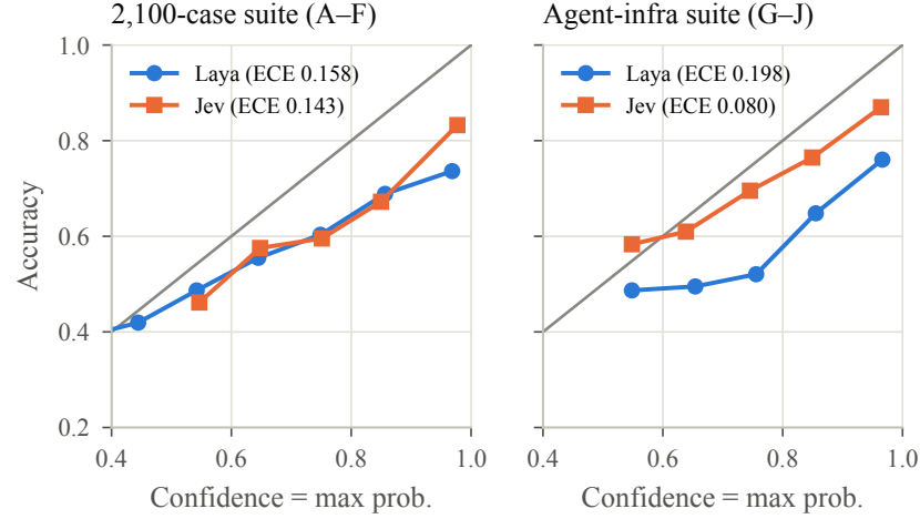
Fig. 7. Reliability diagrams (10 bins, \geq 10 items per point).
