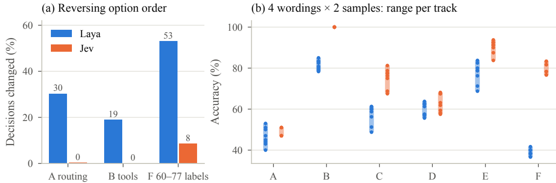
Fig. 3. (a) Share of decisions that change when only the option order is reversed ( n = 1,000 ). (b) Accuracy of each track under 4 instruction wordings \times 2 case samples (600 cases each); dots are the 8 runs.
