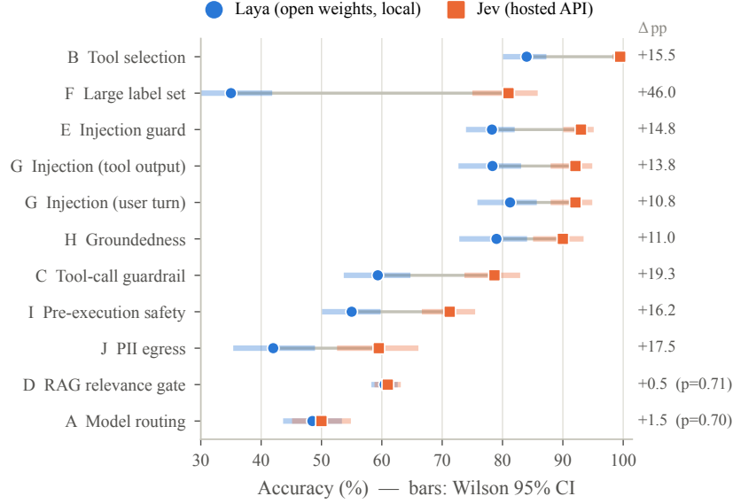
Fig. 1. Accuracy per decision point. Right: paired difference JEV–LAYA (pp); p < 0.001 unless stated.
