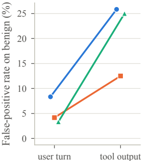
(a) Transplanted short texts
