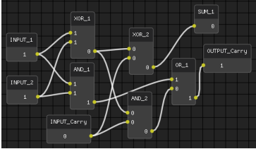
Figure 2: A screenshot of a 1-bit adder network in the C-MCPN Editor.
