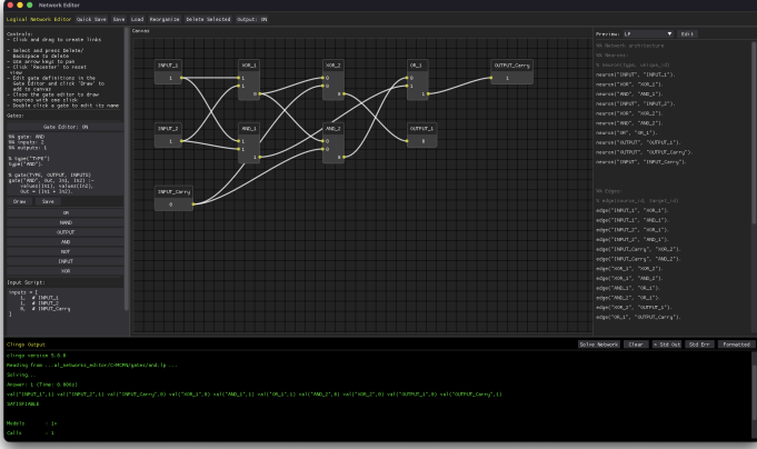
Figure 3: A screenshot of the C-MCPN Editor, showing a sample 1-bit adder network.
