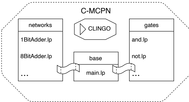
Figure 2: A visualization of the programs involved in the C-MCPN Framework.
