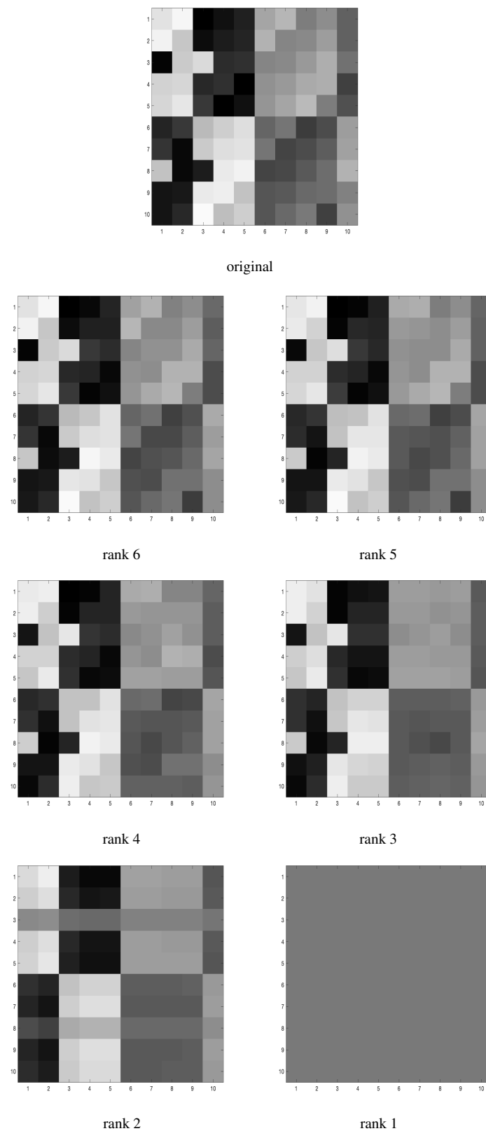
Figure 8.2: The 10-by-10 magic square and its SVD approximations (rank 6 to rank 1), represented graphically. The colour in each square represents the value in the matrix, rescaled to fit in the MATLAB black-and-white colour map.
