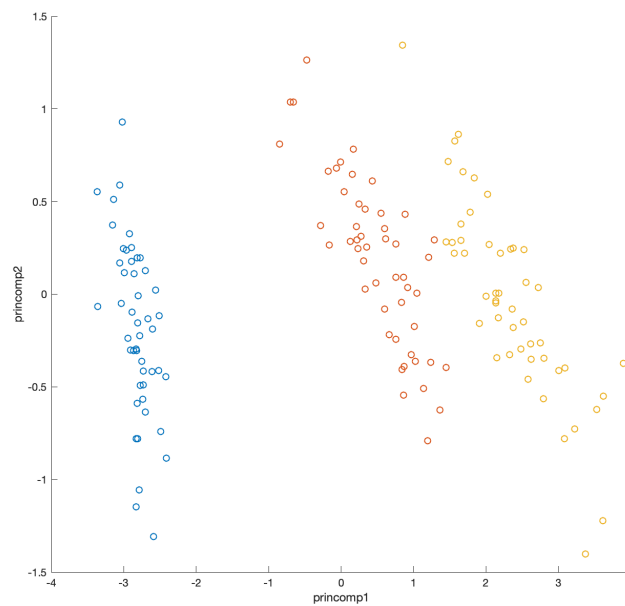
Figure 8.9: Plot of the first and second principal components for the iris data, coloured by species. Now all three species are readily distinguishable, and identifying what species a new data point belonged to would be straightforward.
