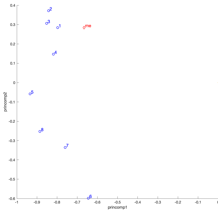
Figure 8.10: Plot of the first and second principal components for the latent semantic indexing approach to identifying nearest neighbours sharing musical preferences. The best matches to me (red diamond) are those users that are nearest.
