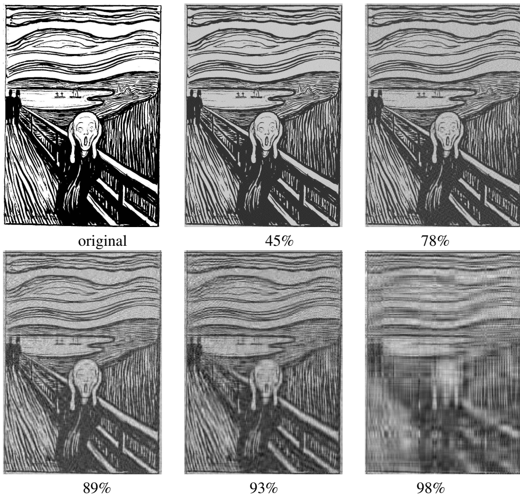
Figure 8.3: Edvard Munch's "The Scream", compressed to various levels (percentage shows reduction of storage data required compared to original) by reducing the rank of the SVD approximation.
