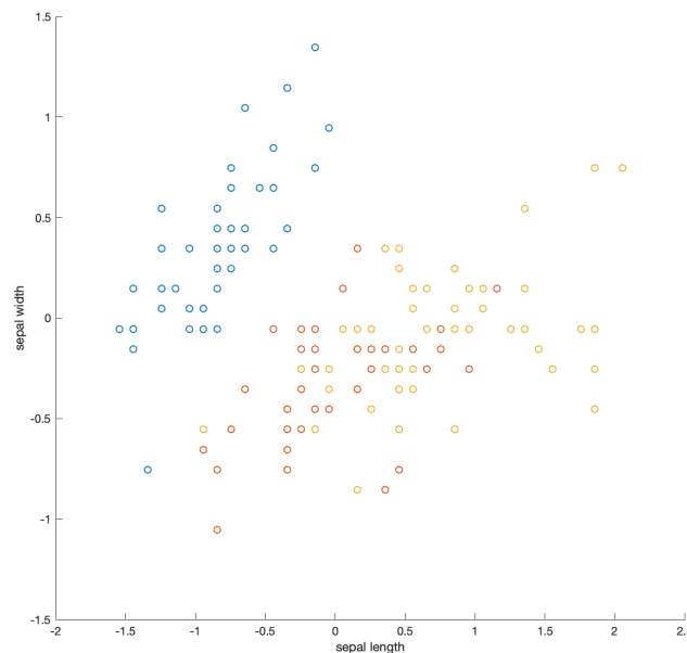
Figure 8.8: Plot of sepal length (horizontal) vs sepal width (vertical) for the iris data, coloured by species. One of the species is readily separable from the others, but the other two have data points that are intermingled. Identifying what species a new data point belonged to would be challenging.
