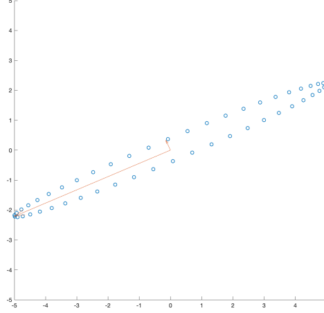
Figure 8.4: Action of multiplying A = \begin{pmatrix} 3 & 4 \\ 1 & 2 \end{pmatrix} on points sitting on the unit circle. We want to figure out the directions of maximum and minimum shrinking, given by the arrows in the figure.
