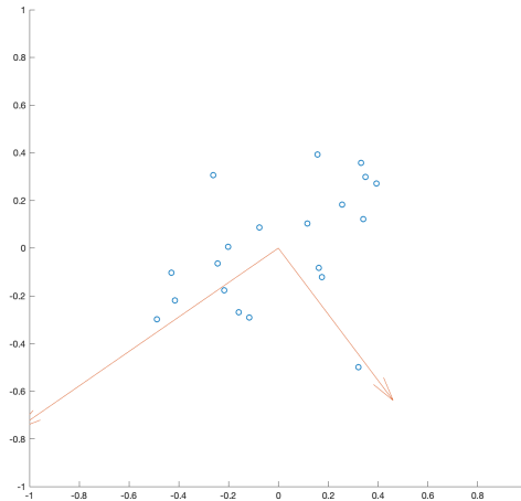
Figure 8.5: Set of 2D data points. We want to figure out the directions of maximum and minimum shrinking, given by the arrows in the figure.
