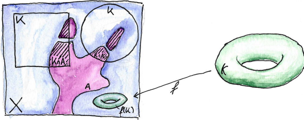
Figure 1: The definition of compactly generated weak Hausdorff spaces.
