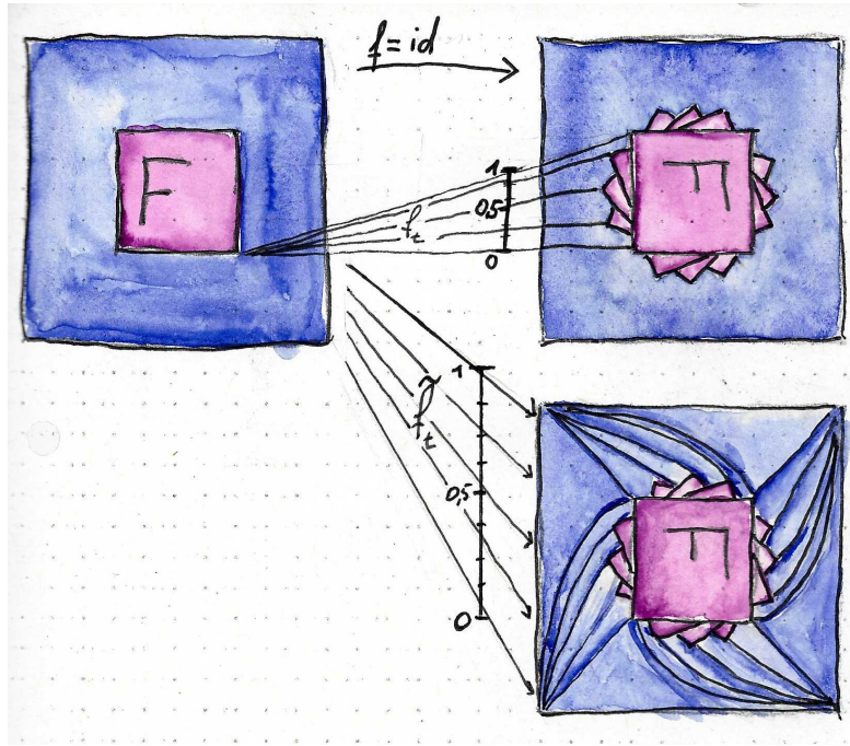
Figure 1: The homotopy extension property for the pair (X, F) , where F gets rotated.
