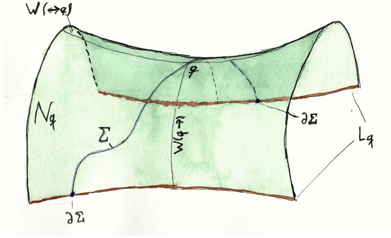
Figure 7: The definition of the transverse \Sigma from Lemma 6.2.9.
