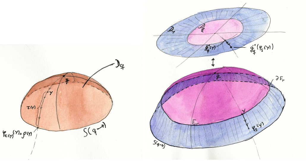
Figure 5: The map \tau and \rho from Lemma 6.2.4 (a) is shown on the left and the map G from (c) is shown on the right.
