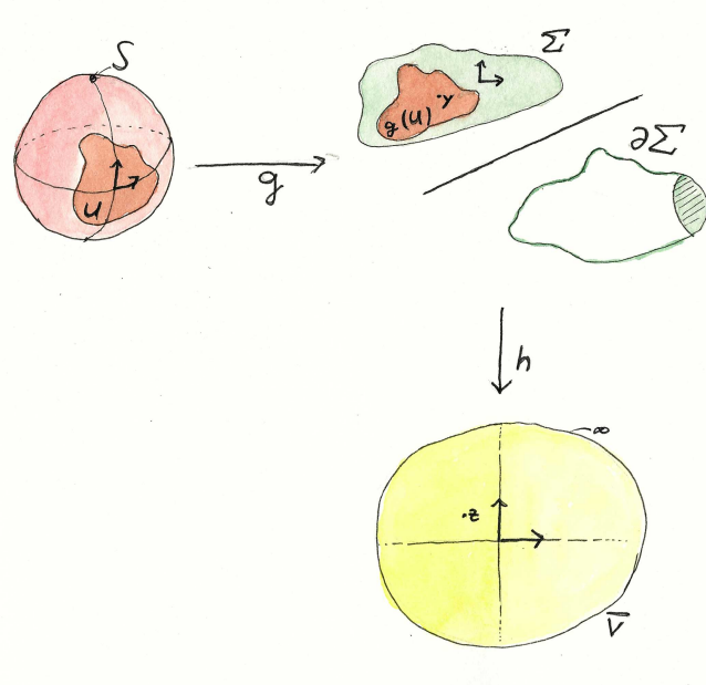
Figure 6: The setup of Lemma 6.2.5.
