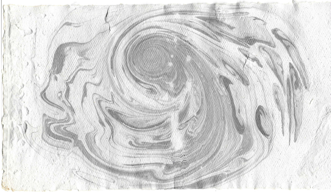
Figure 4: A dynamical system with a critical point created by printing a flow of inc.
