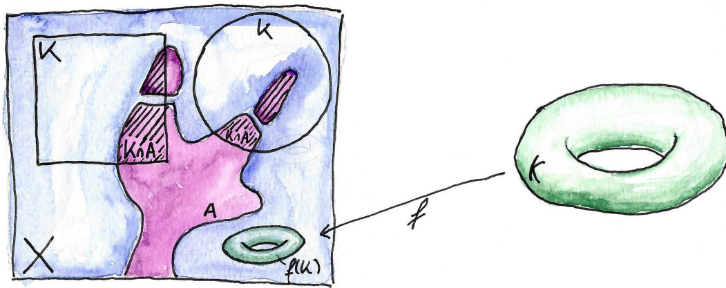
The definition of compactly generated weak Hausdorff spaces.
