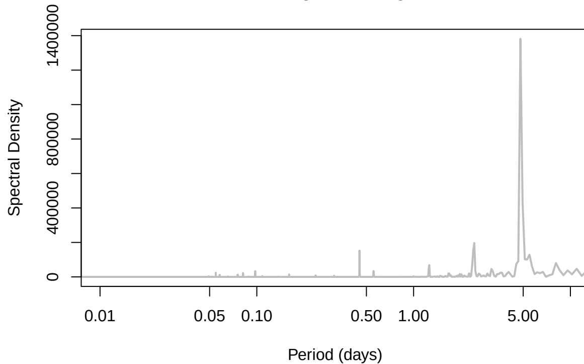
Periodogram – Original
