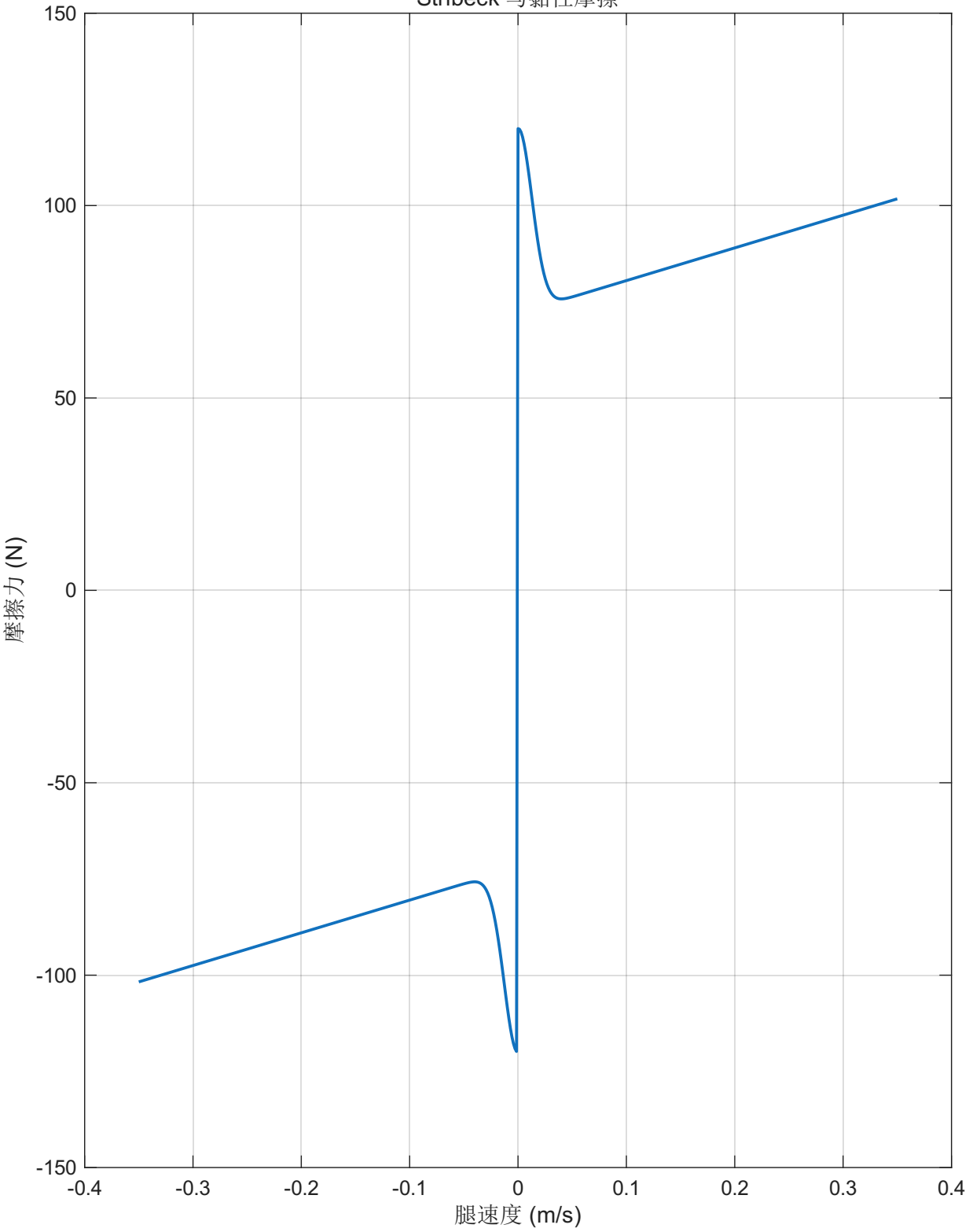
Stribeck 与黏性摩擦
