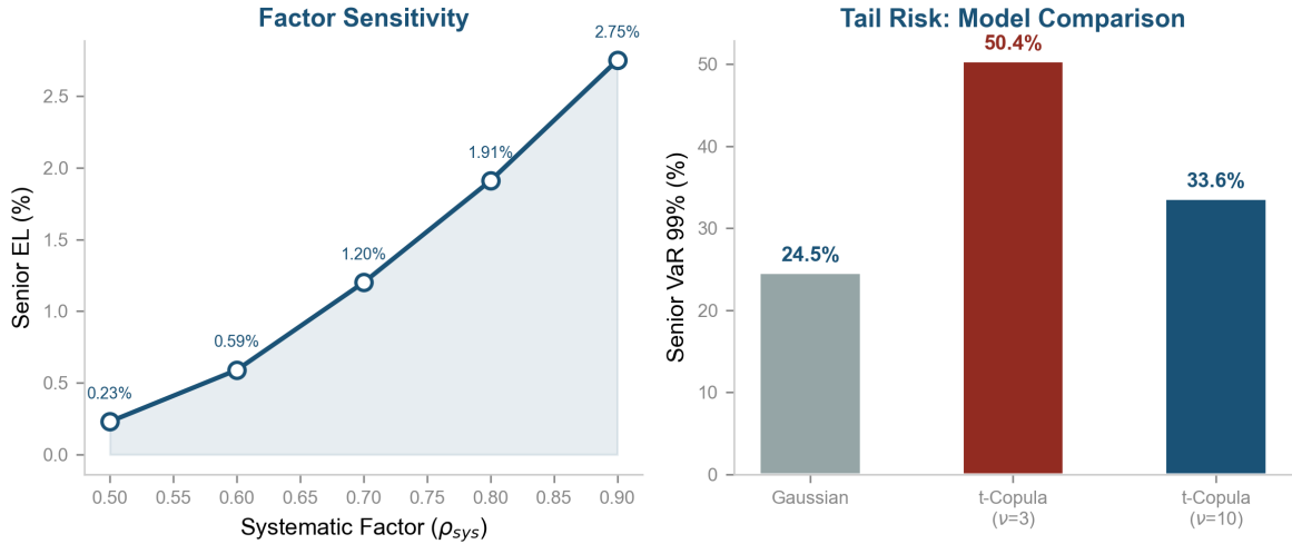
Figure 5: Robustness of Senior tranche losses to model specification. Left: Systematic factor sensitivity \rho_{\text{sys}} \in [0.5, 0.9] . Senior EL ranges from 0.23% to 2.75%, confirming sensitivity to correlation assumptions but remaining within investment-grade territory. Right: Gaussian vs. t -Copula VaR 99%. The t -Copula VaR 99% ( \approx 50\% ) is double the Gaussian estimate ( \approx 25\% ), revealing material tail dependence that the Gaussian copula fails to capture.
