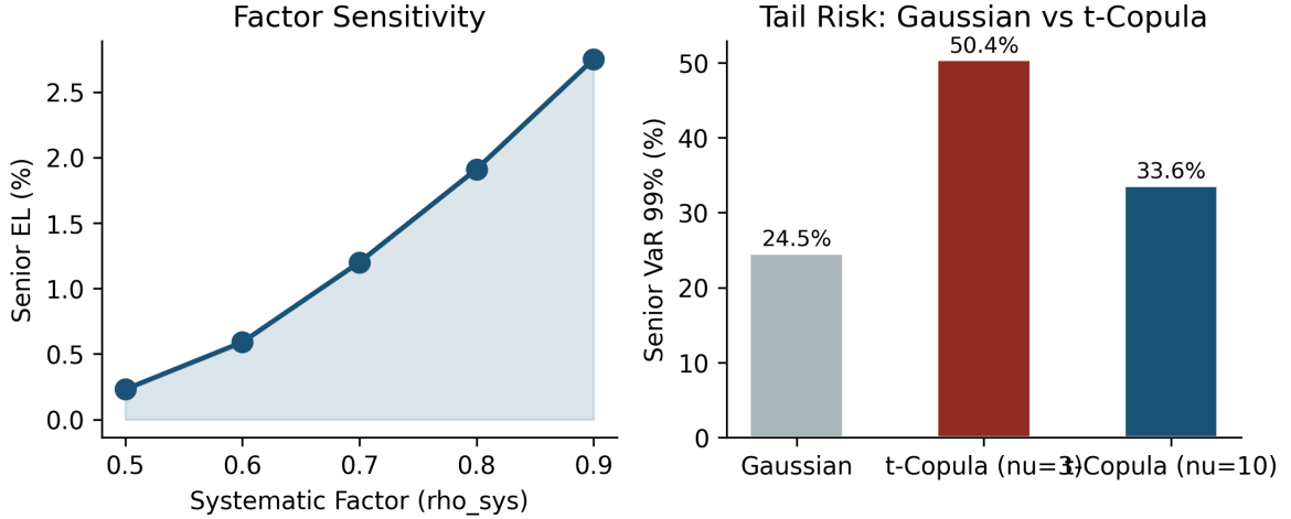
Figure 5: Robustness of Senior tranche losses to model specification. Left: Systematic factor sensitivity \rho_{sys} \in [0.5, 0.9] . Senior EL ranges from 0.23% to 2.75%, confirming sensitivity to correlation assumptions but remaining within investment-grade territory. Right: Gaussian vs. t -Copula VaR 99%. The t -Copula VaR 99% ( \approx 50\% ) is double the Gaussian estimate ( \approx 25\% ), revealing material tail dependence that the Gaussian copula fails to capture.
