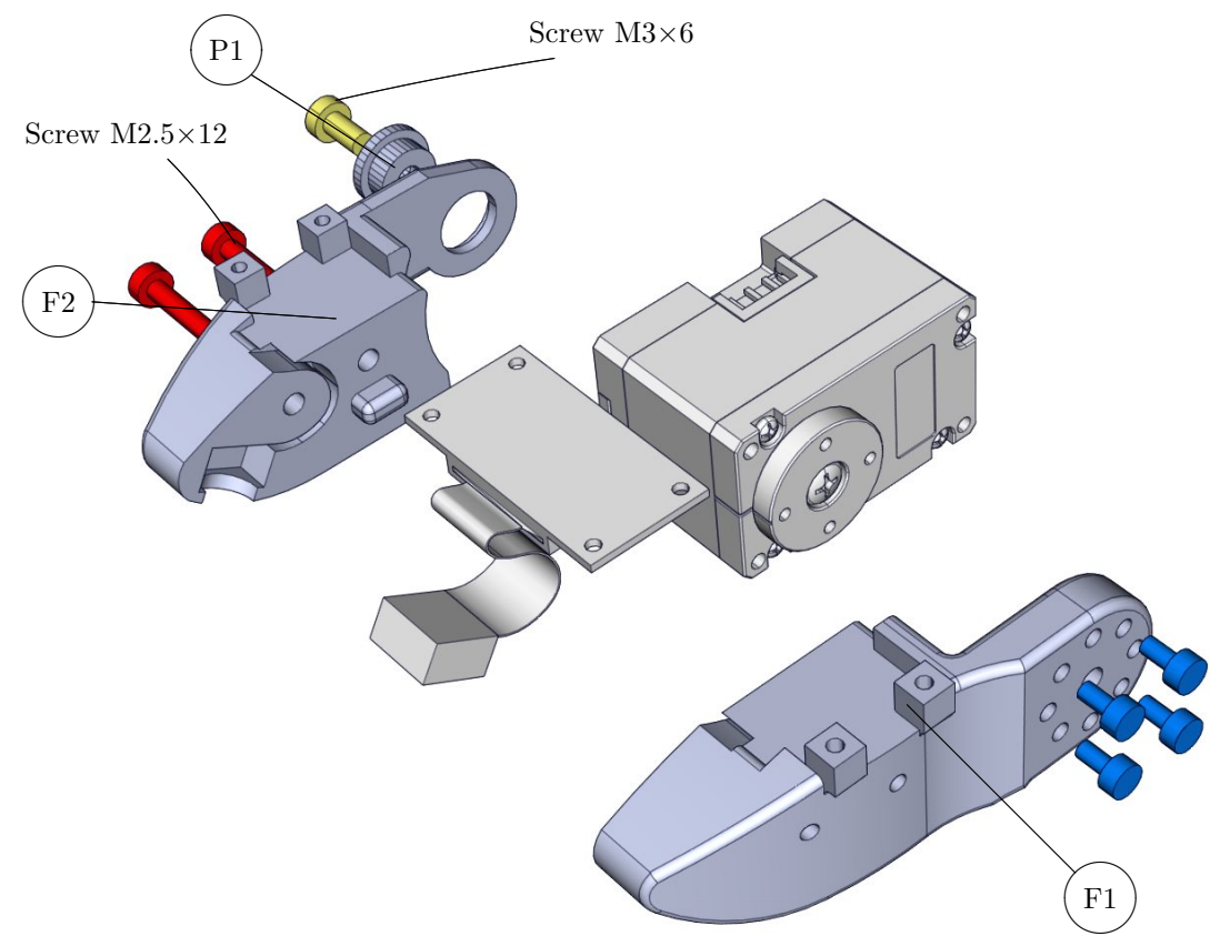
Exploded View
