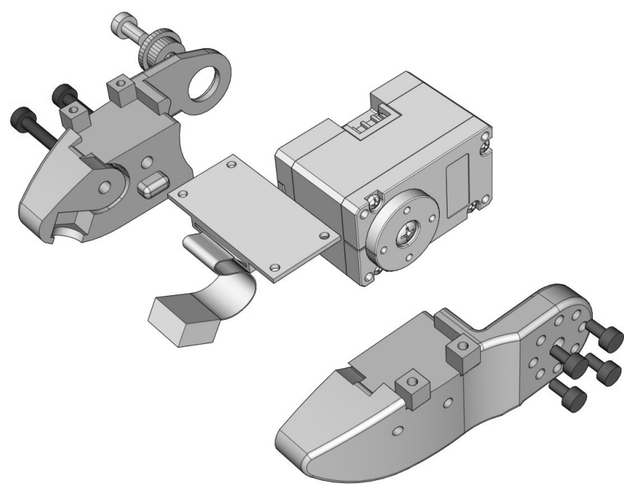
Exploded View
