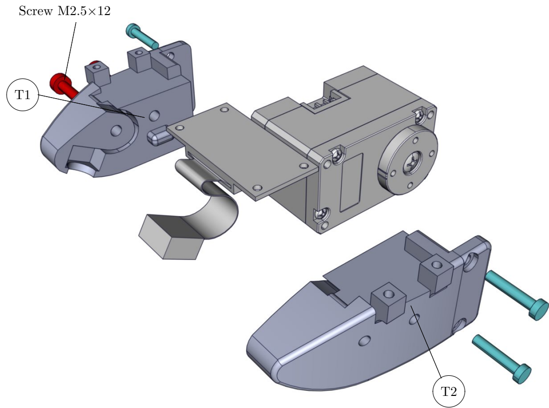
Exploded View
