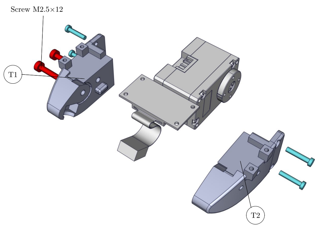
Exploded View
