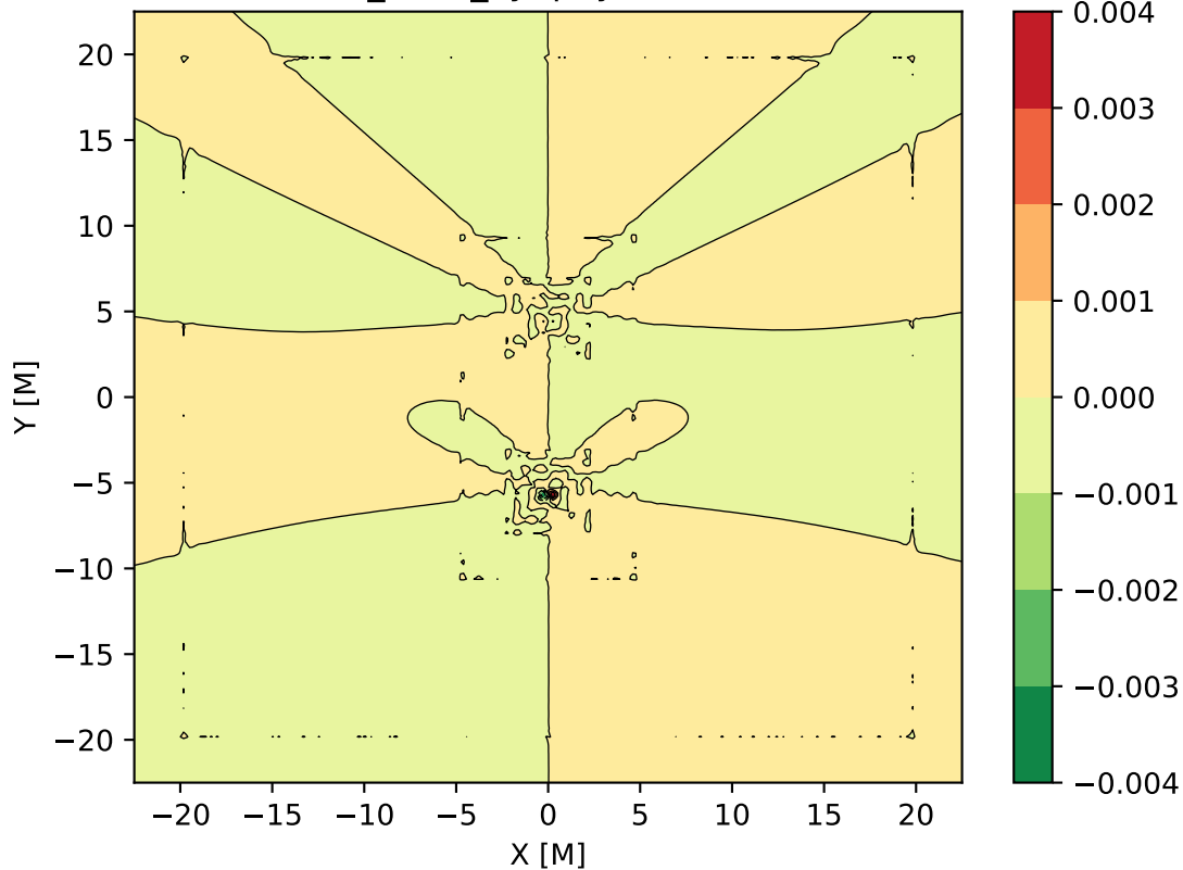
Lev04-00_Cons_Py physical time = 0.0
