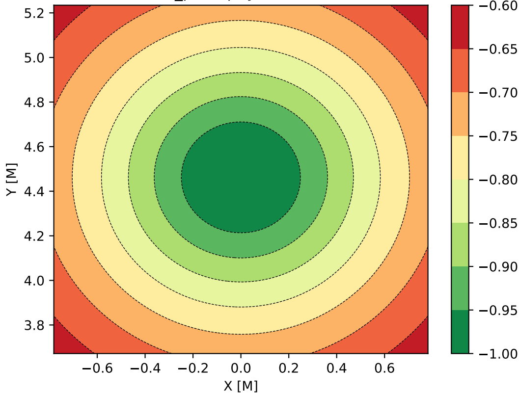
Lev08-00_phi0 physical time = 0.0
