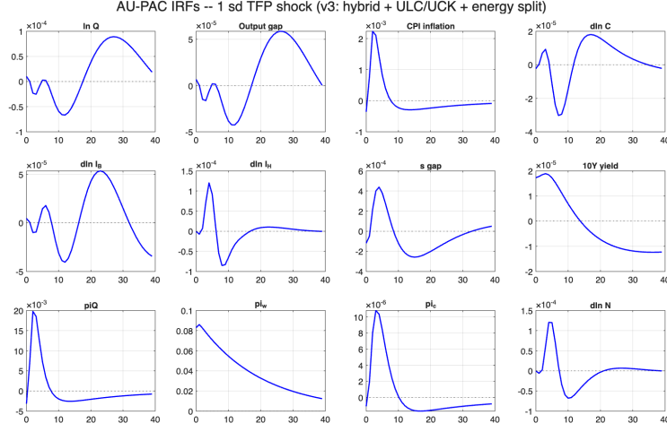
Figure 11: TFP shock
