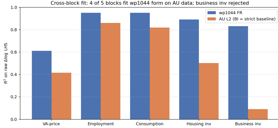
Figure 4: Cross-block R²: 4 of 5 blocks fit wp1044 form on AU data
