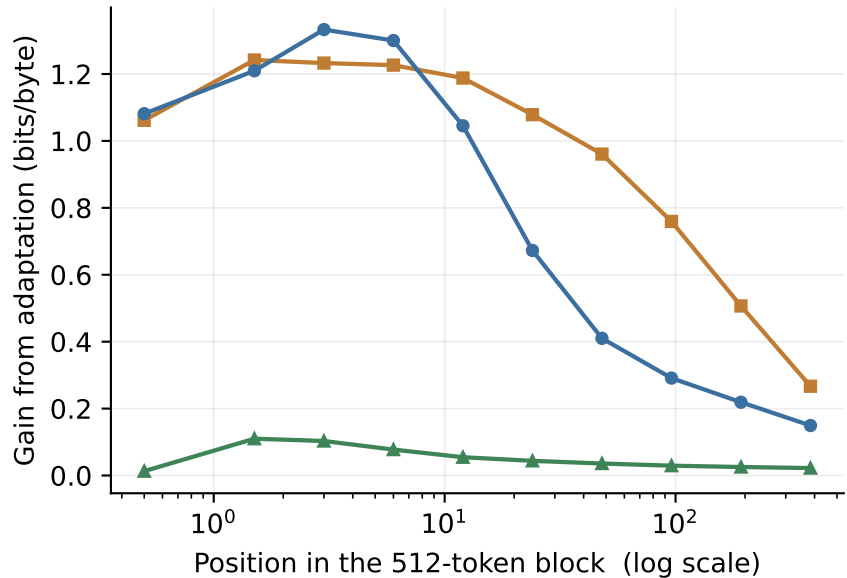
Loss reduction from adaptation
