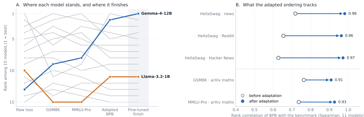
Figure 1: What adaptation does to the ordering of base models. A: rank of each of the fifteen fine-tuned models under raw (unadapted) loss, GSM8K, MMLU-Pro and adapted BPB, beside where its system finishes after fine-tuning on a news task. Gemma-4-12B is thirteenth on raw loss and mid-table on both benchmarks, second by adapted BPB, and builds the best system of all; Llama-3.2-1B is last on both benchmarks and finishes eleventh, exactly where adapted BPB places it. B: rank correlation between BPB and each benchmark over the eleven-model cohort, before adaptation (hollow) and after (filled). Adapted on general text, the ordering converges on HellaSwag on all three corpora; adapted on arXiv mathematics, it swings to the reasoning benchmarks.
