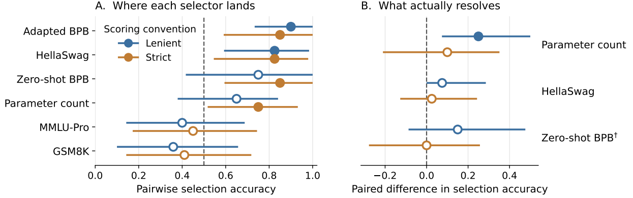
Figure 5: How often each way of choosing a base model agrees with the news quiz. Seventeen models, the 40 pairs within 2\times of each other in size, judged by the news quiz (Section B; lenient unless marked strict). A: each selector’s accuracy. Adapted BPB is top under lenient scoring and level with the unadapted reading under strict; both generative benchmarks fall below chance by point estimate. B: adapted BPB’s accuracy minus each alternative’s on the same pairs, so positive favours adapted BPB. Intervals are 95% cluster-bootstrap over models; a hollow marker means the interval still contains chance (A) or zero (B). One comparison resolves at this cohort size: adapted BPB over parameter count, +0.250 [+0.074, +0.500] , lenient. † computed after the fact rather than preregistered.
