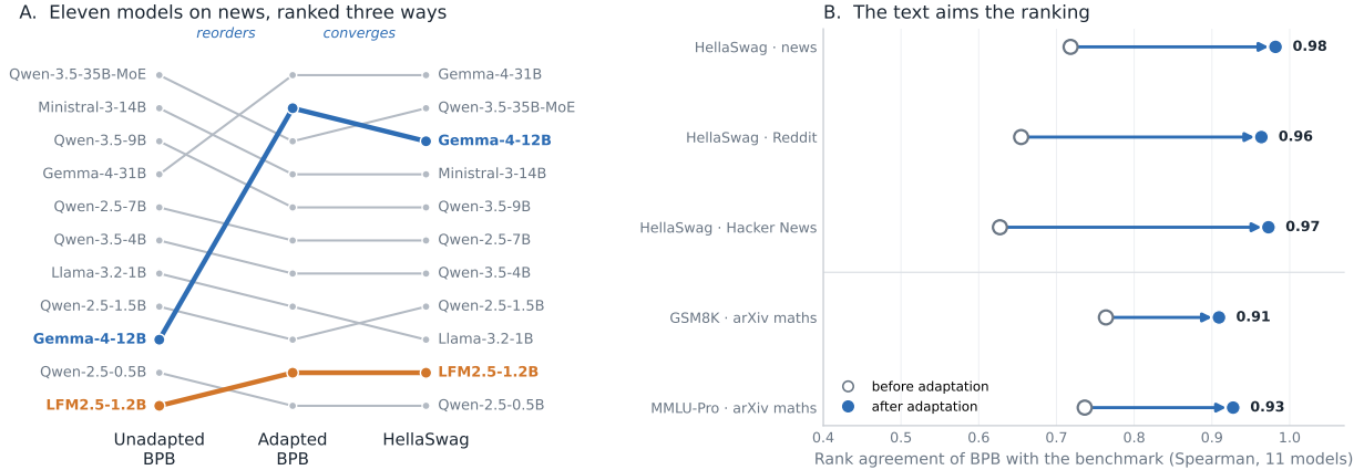
Figure 1: Adaptation reorders the models, and the text aims the new order. A: the eleven models evaluated on all four corpora, ranked by unadapted news bits per byte (BPB; lower is better), by adapted news BPB and by HellaSwag. Between the first two columns the lines cross: adaptation reorders the models, lifting Gemma-4-12B from ninth to second and LFM2.5-1.2B out of last place. Between the last two they run almost parallel: the adapted order is HellaSwag’s. B: rank agreement (Spearman \rho , signed so that 1 means lower BPB goes with a higher score) between BPB and each benchmark, before adaptation (hollow) and after (filled). Adapted on general text, the ranking converges on HellaSwag on all three corpora; adapted on arXiv mathematics, it turns to GSM8K and MMLU-Pro. The full matrix is Table 4 in Appendix B.
