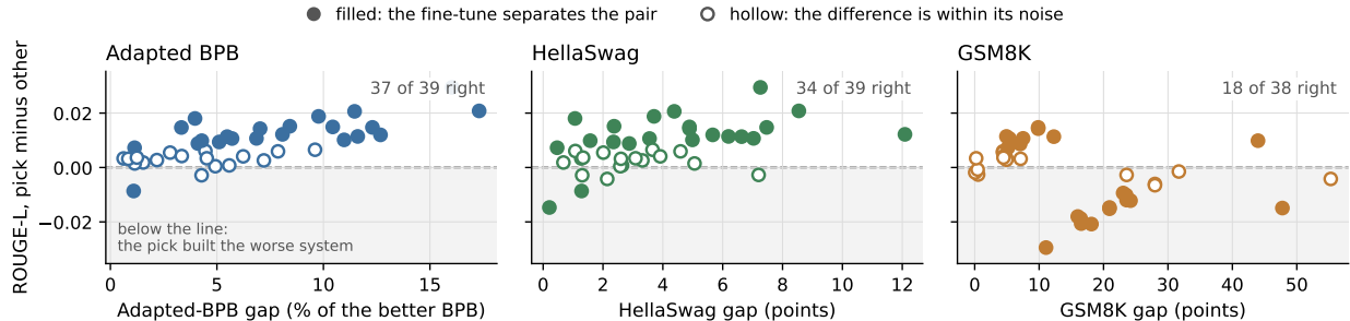
Figure 3: Does each way of ranking agree with the fine-tuned outcome? Each point is one pair of the fifteen fine-tuned models whose parameter counts are within 2\times of each other: 39 such pairs, 38 for GSM8K, on which two models tie. Each pair is oriented so that the ranking prefers its first model: x is how strongly it prefers it (the gap in that measure), y is how much higher the first model’s fine-tuned system scores in ROUGE-L. Points above the line are pairs the ranking orders as the fine-tune does; filled markers are resolved pairs, whose ROUGE-L difference has a 95% bootstrap interval over the 500 articles that excludes zero. Adapted BPB agrees on 37 of 39, and on 21 of the 22 resolved pairs; HellaSwag on 34; GSM8K on 18 of 38, and every one of its eleven gaps between 15 and 25 points sits below the line.
