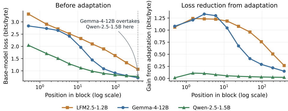
Figure 4: Why the unadapted number mis-ranks: it mostly measures how fast a model settles into unfamiliar text. Each evaluation block starts with no earlier context, so every block begins cold. Left : unadapted loss by position within a packed 512-token evaluation block, for Gemma-4-12B, Qwen-2.5-1.5B and LFM2.5-1.2B. Unadapted, Gemma-4-12B opens a block at 2.83 bits per byte against Qwen-2.5-1.5B’s 2.04 (a 12B model losing to a 1.5B one) and closes it at 0.72 against 0.77. A block average over-weights the opening, and that is part of what puts Gemma-4-12B ninth of eleven on unadapted BPB. Right : the loss reduction adaptation buys at each position is largest in the opening but does not vanish after it: adaptation teaches the corpus’s opening conventions, and does more besides. The right panel uses the three adapters of the earlier per-model search (Appendix C), so its gains differ from the fixed-recipe ones in Table 2; the pattern by position is what it shows.
