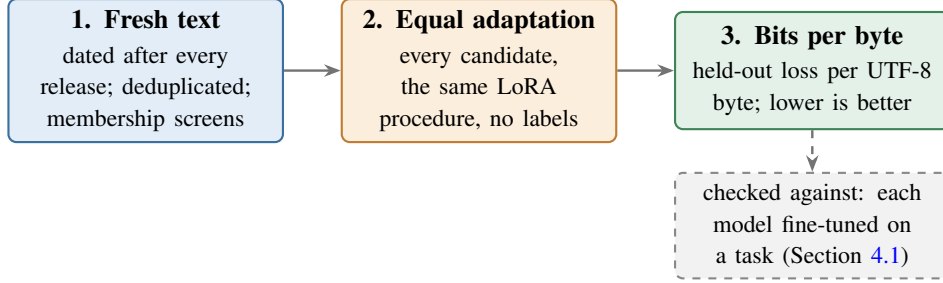
Figure 2: The method. The corpus is fixed and screened first, then every candidate is adapted the same way and scored on held-out text. The fine-tune of Section 4.1 is not part of the measurement; it is what the measurement is checked against.
