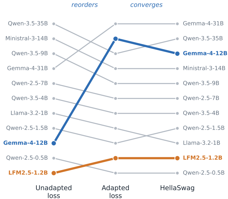
A. Eleven models on news, ranked three ways
