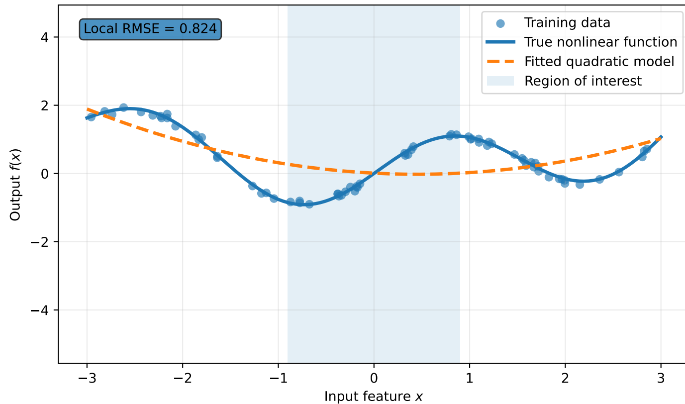
A. Data distributed across the full domain
