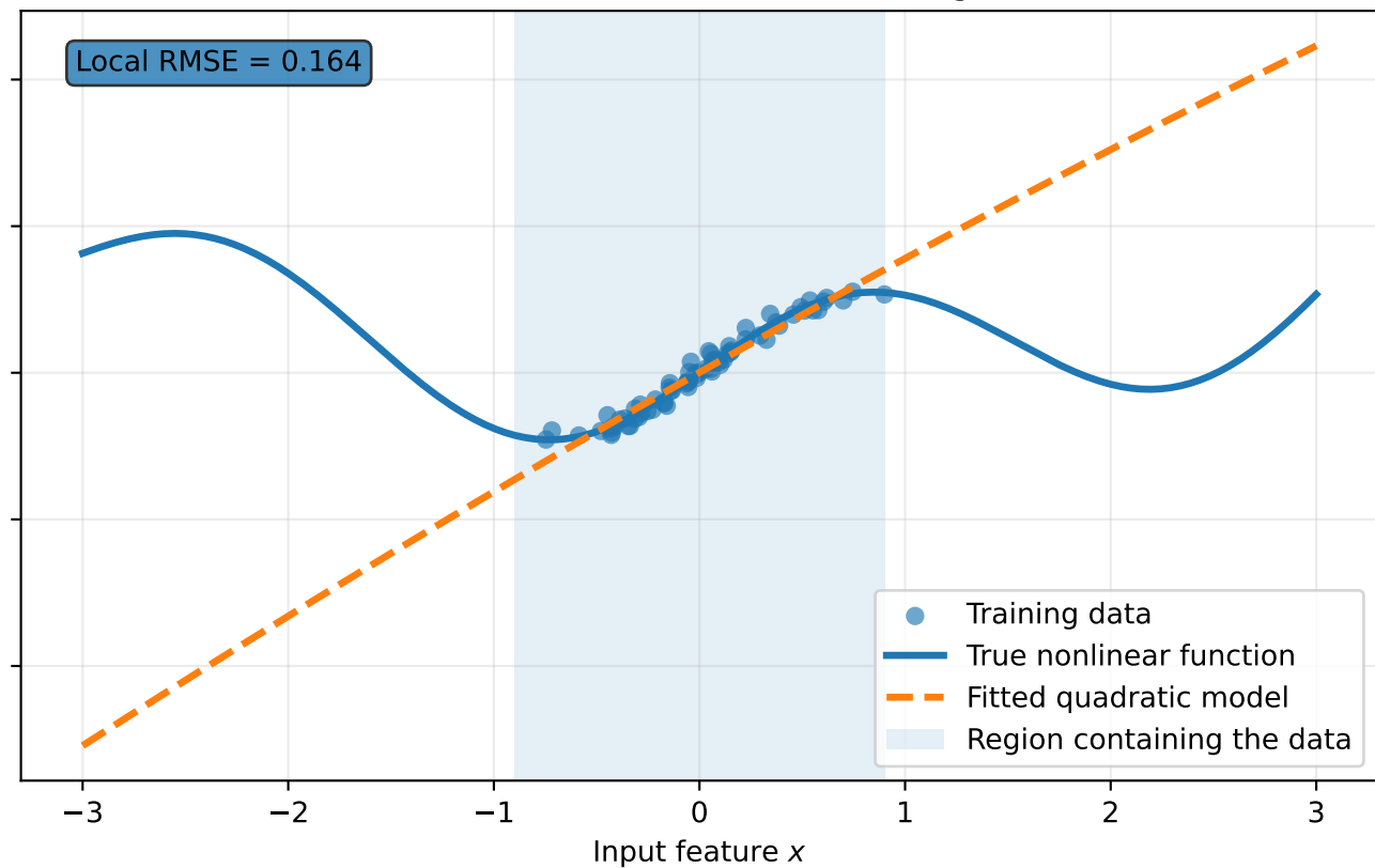
B. Data concentrated in a local region
