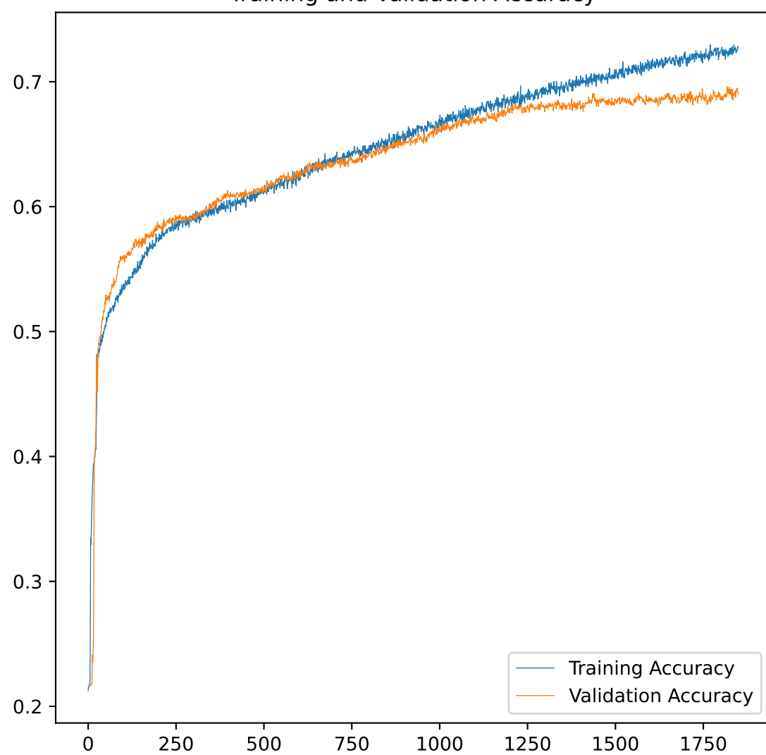
Training and Validation Accuracy
