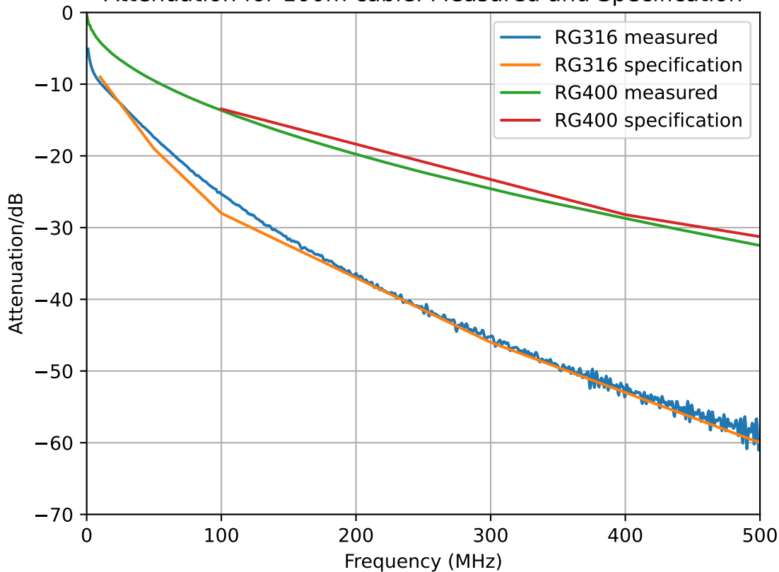
Attenuation for 100m cable. Measured and Specification
